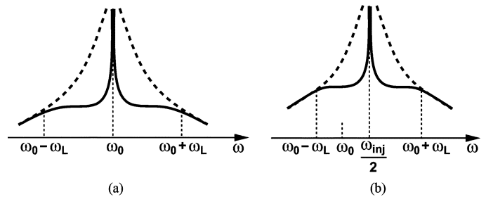
Fig. 1. Phase noise degradation in an ILD.
