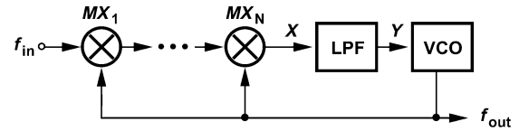
Fig. 4. Heterodyne PLL.
