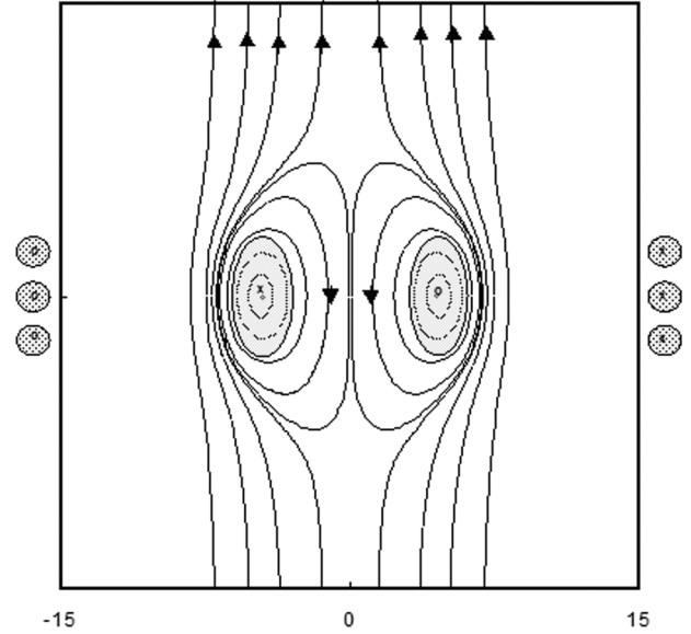
Fig. 9. Detached current ring and its B field in a plasma. Field of the external antenna has been added to that generated by the current ring [1]. Assumed conditions: n = 8 \times 10^{10} \text{ cm}^{-3} plasma with p = 10 mTorr, kT_e = 3 eV, and f = 2 MHz.
