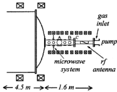
Fig. 17. Helicon experiment of Kline et al. [38]. Measurements were made in port A downstream from the source region.
