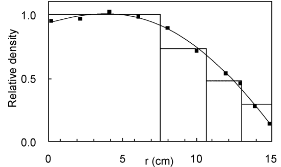
Fig. 6. Histogram of the density distribution of Fig. 5, together with the experimental curve of Fig. 1 [1].
