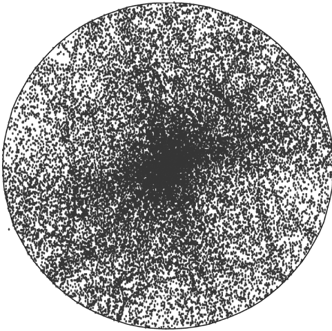
Fig. 5. Distribution of electron positions after 32 000 2-ns time steps [1].
