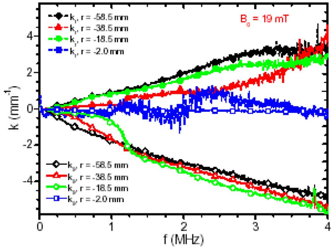
Fig. 23. Propagation constants k_r and k_\theta of the low-frequency wave [41]. (Color version available online at http://ieeexplore.ieee.org .)
