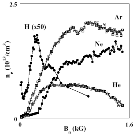
Fig. 10. Helicon density on axis for various gases versus magnetic field [32].
