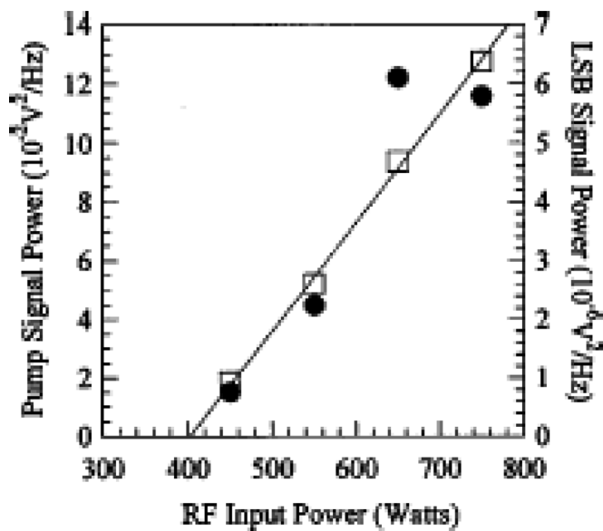
Fig. 19. Power in the pump ( \square ) and the lower sideband ( \bullet ) versus input power [38].
