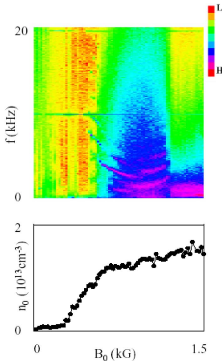
Fig. 11. Bottom: density versus B_0 measured in neon. Top: frequency spectrum of probe signals on same scale [32]. (Color version available online at http://ieeexplore.ieee.org .)
