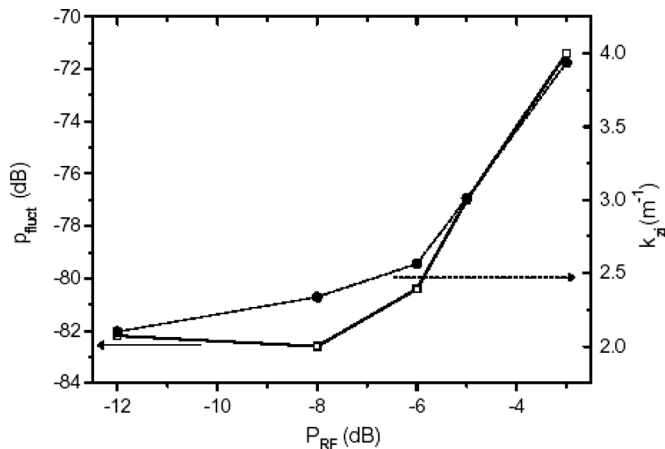
Fig. 26. Nonlinear increase of low-frequency power and helicon damping [41].
