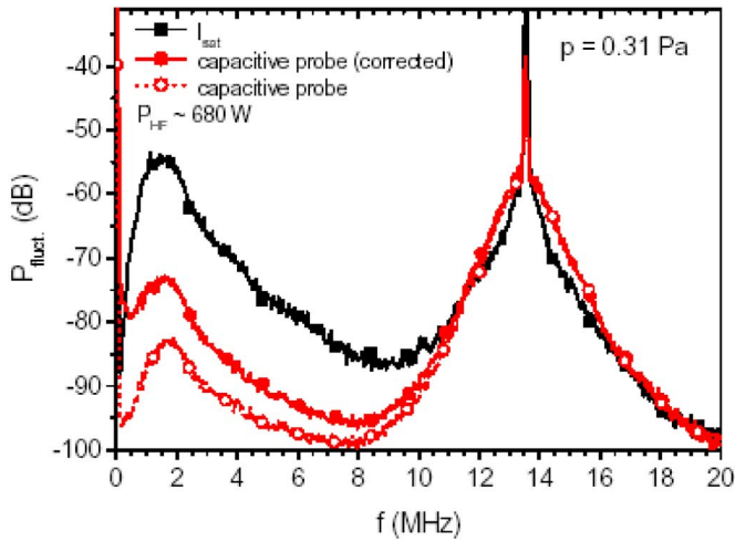
Fig. 22. Frequency spectra taken with electrostatic (top curve) and capacitive (middle curve) probes. Bottom curve is uncorrected for the frequency response of the capacitive probe [41]. (Color version available online at http://ieeexplore.ieee.org .)
