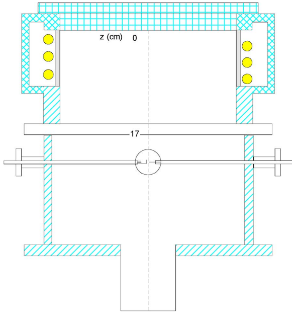
Fig. 2. Schematic of a commercial processing reactor with a side-mounted antenna. (Color version available online at http://ieeexplore.ieee.org .)
