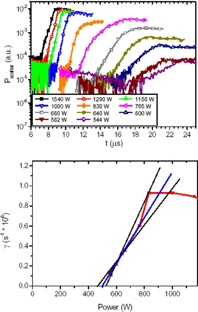
Fig. 25. Direct measurements of wave growth using microwave backscatter at various RF powers. Bottom graph shows the measured growth rates compared with the theoretically computed range [41]. (Color version available online at http://ieeexplore.ieee.org .)
