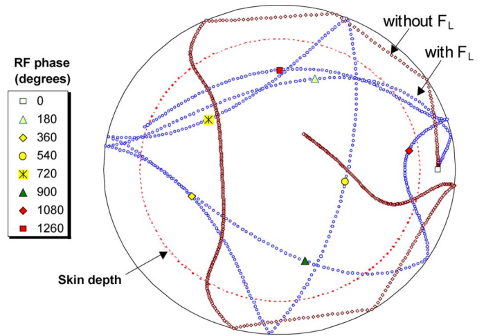
Fig. 3. Trajectory of an electron through four RF cycles [1]. Assumed parameters: f = 6.78 MHz, skin depth = 3.1 cm, tube radius = 15 cm, sheath drop = 20 V, p = 10 mtorr (argon), and KT_e = 3 eV. (Color version available online at http://ieeexplore.ieee.org .)
