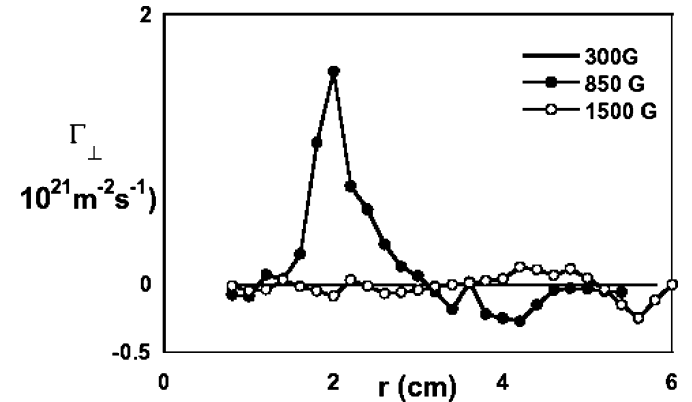
Fig. 13. Measured radial flux versus radius at three magnetic fields [33].
