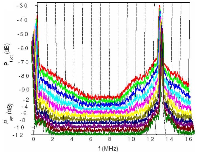
Fig. 21. Electrostatic-probe spectra at various RF powers, increasing upwards [41]. (Color version available online at http://ieeexplore.ieee.org .)
