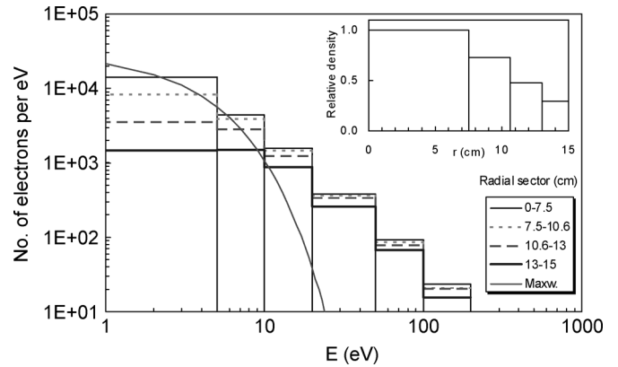
Fig. 7. Calculated energy distributions in each sector, compared with a Maxwellian (curve), on a log-log scale. Radii covered by each sector are shown in the inset [1].
