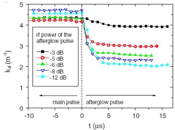
Fig. 20. Axial damping rate \text{Im}(k_z) versus time, showing an increase with P_{\text{RF}} [41]. These pulsed experiments were done with P_{\text{RF}} \leq 2 kW at 13.56 MHz, p = 1.5 –4.5 mtorr, B_0 \leq 1000 G, yielding n \leq 2 \times 10^{13} \text{cm}^{-3} and K T_e \approx 3 eV. (Color version available online at http://ieeexplore.ieee.org .)
