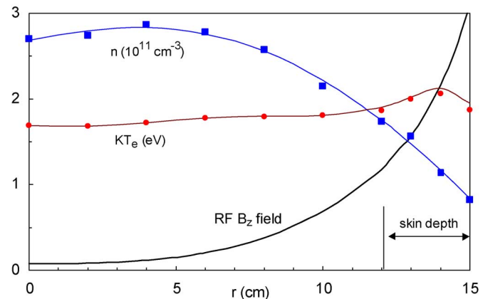
Fig. 1. Radial profiles of density, electron temperature, and the RF B_z field in the apparatus of Fig. 2 [1]. (Color version available online at http://ieeexplore.ieee.org .)
