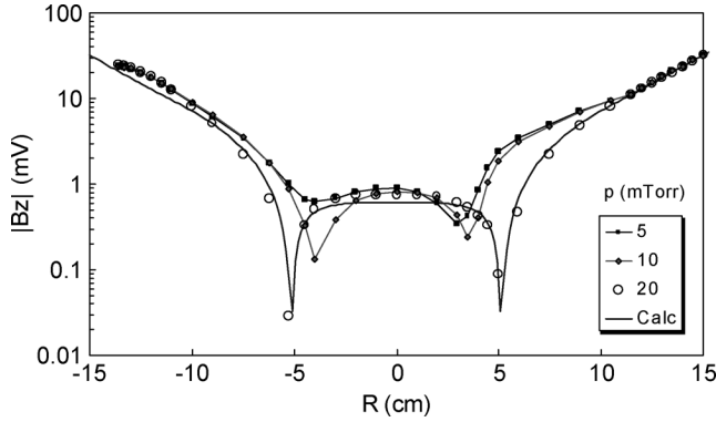
Fig. 8. Radial profiles of RF B_z field at various pressures. Bottom curve is a computed fit to the 20-mTorr data [1]. Experimental conditions: 400 W at 2 MHz, 5–20 mTorr of Ar.
