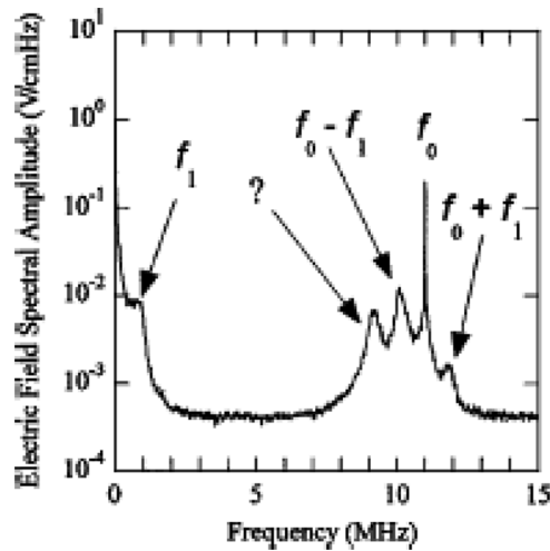
Fig. 18. Spectrum of electrostatic oscillations [38].
