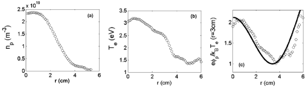
Fig. 14. Density, T_e , and normalized space potential versus radius [35].
