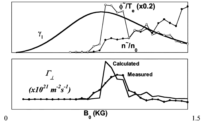
Fig. 12. Top: computed growth rate versus B_0 compared with measured potential and density fluctuation amplitudes. Bottom: calculated and measured radial transport fluxes [33].
