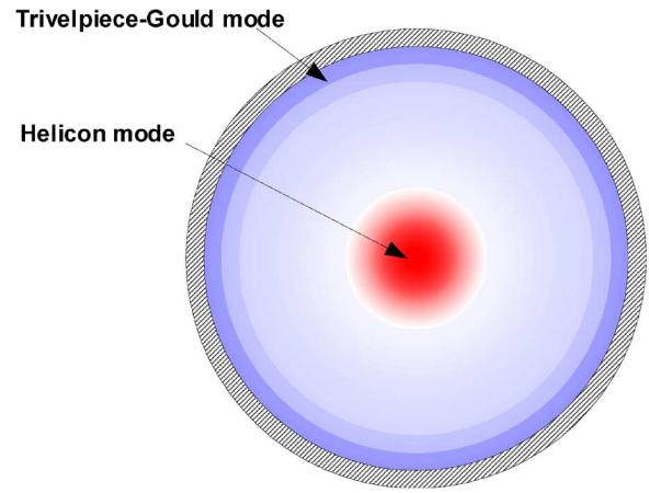
Fig. 16. Illustration of the coupled helicon and Trivelpiece-Gould waves. (Color version available online at http://ieeexplore.ieee.org .)
