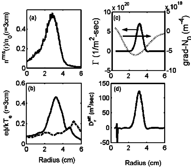
Fig. 15. Radial profiles of (a) normalized density fluctuations, (b) normalized potential fluctuations, (c) radial flux from correlations with the density gradient, and (d) computed diffusivity [35].
