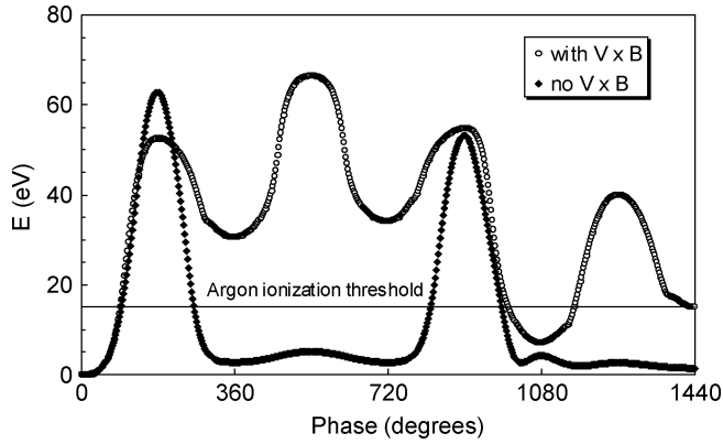
Fig. 4. Energy of the test electron computed with (○) and without (◆) the Lorentz force, for an applied RF E field of 8 V/cm at 6.78 MHz [1].
