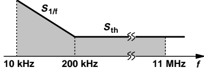
Fig. 7. Contribution of flicker noise to the overall SNR .
