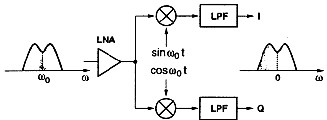
Fig. 3. Direct-conversion architecture.
