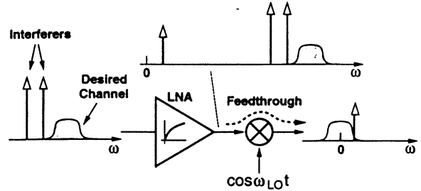
Fig. 8. Effect of even-order distortion on interferers.
