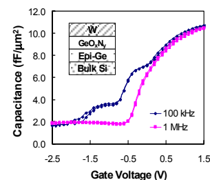
Figure 3. Bi-directional CV characteristics of epi-Ge MOS capacitors with GeO x N y gate dielectric and W gate electrode: 100 kHz and 1 MHz.
