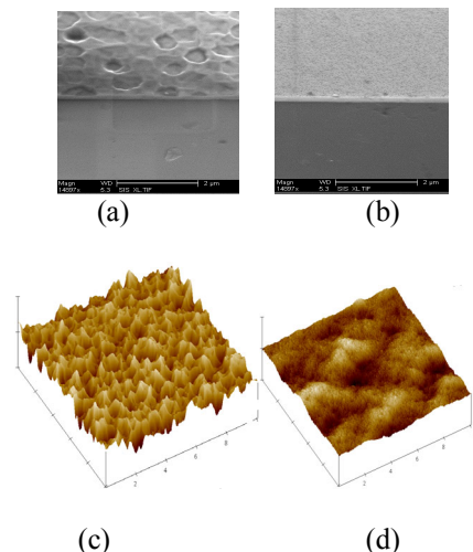
Figure 1. Cross section HR-SEM image of (a) No anneal (b) 825°C H 2 anneal; Surface AFM image of epi-Ge layer: (10μm X 10μm) (c) No anneal, (d) 825°C H 2 anneal.
