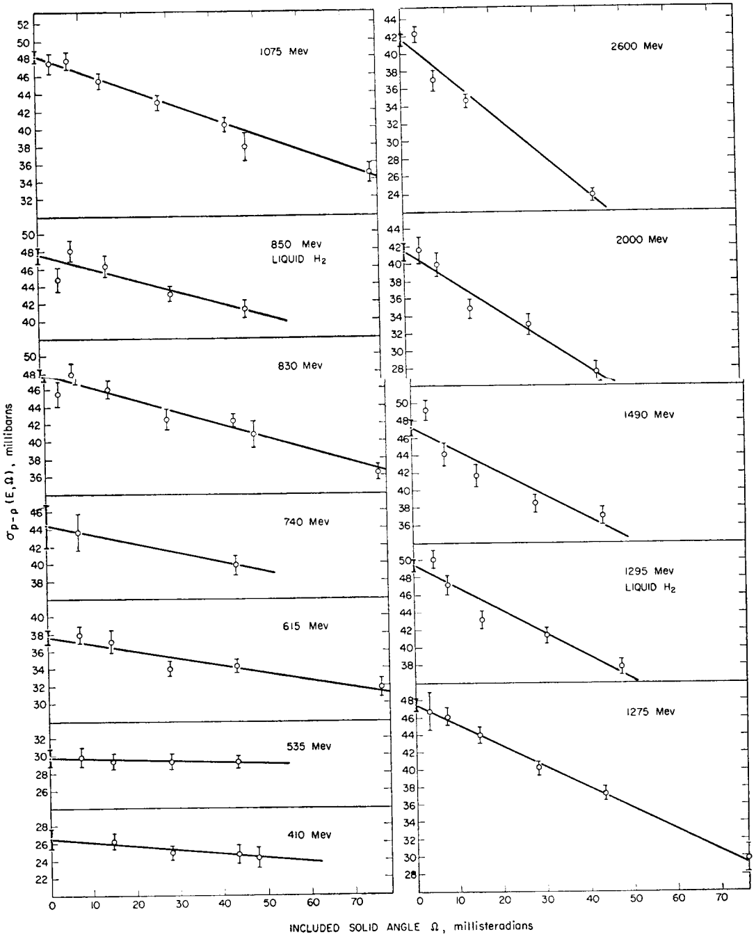
FIG. 4. The measured values of \sigma_{p-p}(E, \Omega) , corrected for multiple Coulomb scattering, plotted as a function of the included solid angle \Omega for the various proton kinetic energies E that were studied. The straight lines were fitted to the data by least squares calculations.
