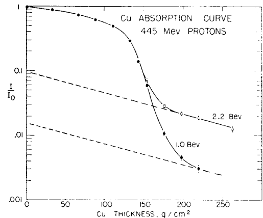
Fig. 2. Integral range curves in copper of the 445-Mev proton beam. The upper curve was obtained with the Cosmotron operating at an energy of 2.2 Bev, and the lower curve at 1 Bev. The extrapolations shown were made using a geometric cross section of \pi(1.254 \times 10^{-13})^2 \text{ cm}^2 .
