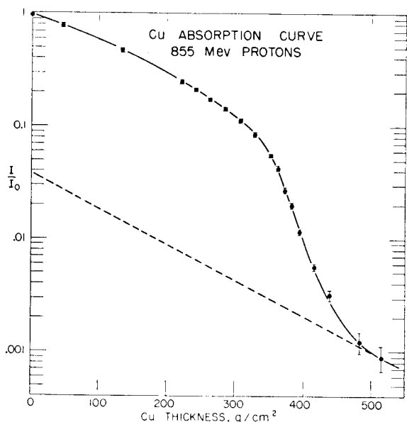
FIG. 3. Integral range curve in copper of the 855-Mev proton beam with the Cosmotron operating at an energy of 2.2 Bev. The extrapolation shown was made using a geometric cross section of \pi ( 1.25 \cdot 10^{-19} ) 2 cm 2 .
