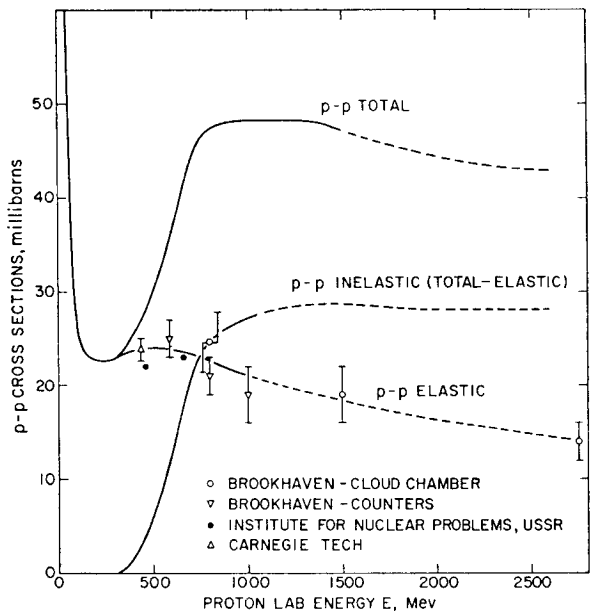
FIG. 8. The total, elastic, and inelastic p-p cross sections as a function of proton energy. The plotted points all represent measurements of the elastic p-p cross section. The inelastic curve (except below 440 Mev) was obtained by subtracting the elastic curve from the total p-p curve. References: Brookhaven cloud chamber—reference 23; Brookhaven counters—reference 9; Institute for Nuclear Problems, U.S.S.R.—references 24 and 27; Carnegie Tech—reference 1.
