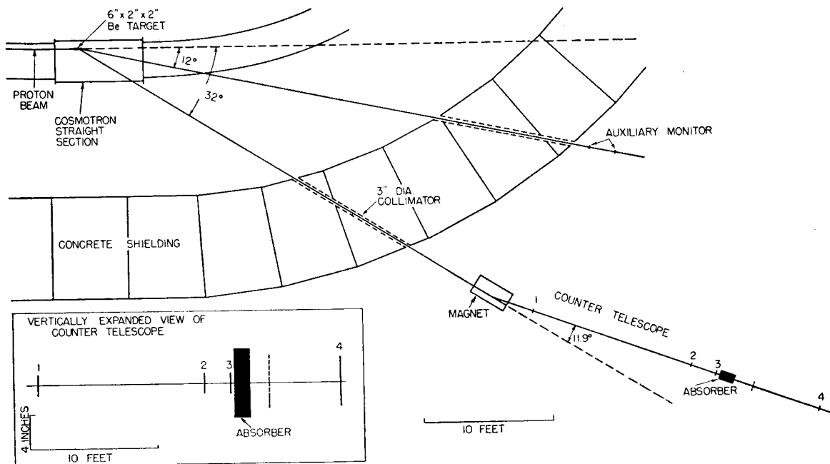
FIG. 1. Experimental arrangement.
