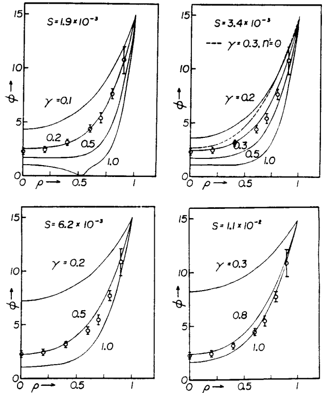
FIG. 4. The theoretical potential profiles \phi(\rho) in comparison with the experimental points, for various values of \gamma , and for values of S corresponding to kT_i = 0.1, 0.3, 1, and 3 ev.
