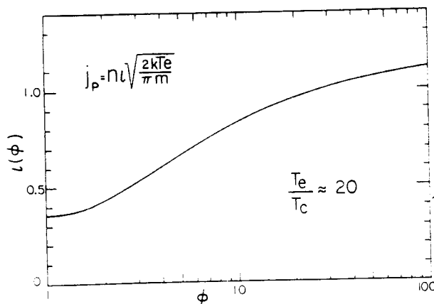
FIG. 3. Space-charge-limited emission in a plasma as a function of sheath drop.
