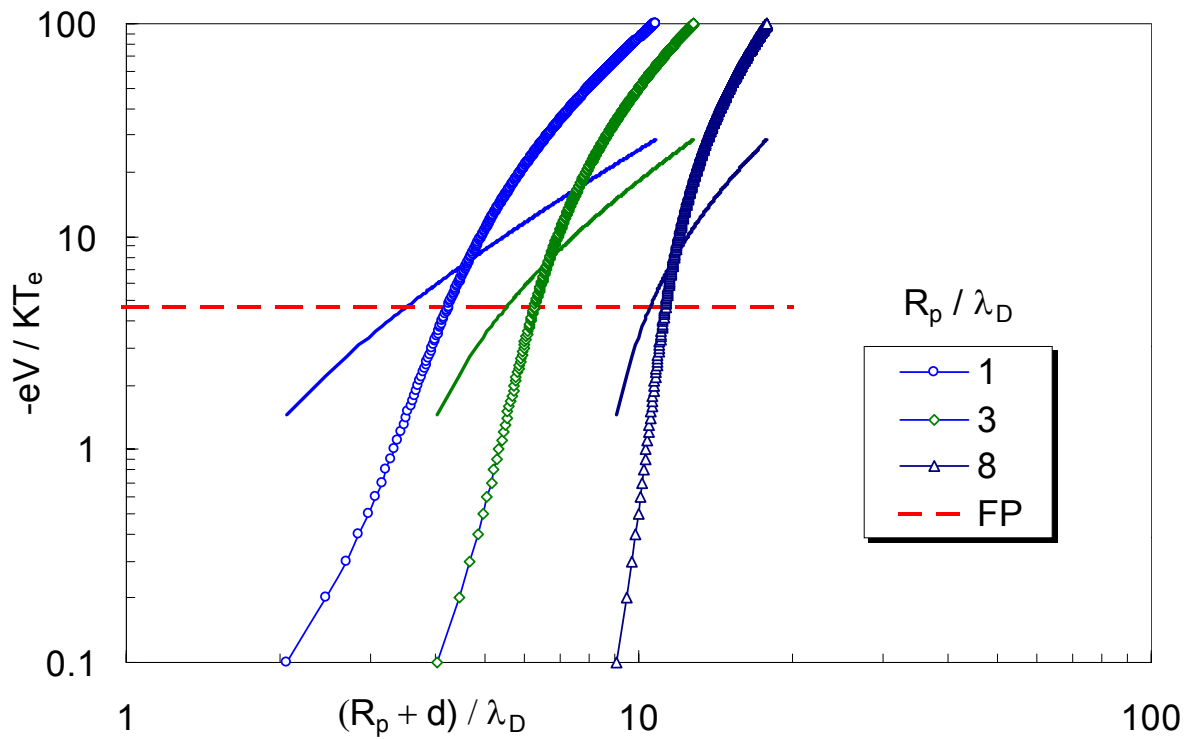
Fig. 8. Normalized sheath radii for various values of R_p/\lambda_D as calculated (points) and as estimated with the CL formula (lines). The right-hand curve of Fig. 7 was used. The dashed line is the floating potential.
