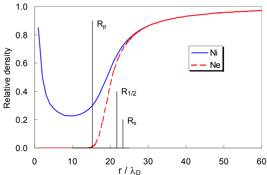
Fig. 16. ABR solution for the ion (—) and electron (---) densities in the sheath for the case J = 10 . The radius of a floating probe is shown by the line labeled R_p . Similarly, R_{1/2} is the radius where \eta = 1/2 , and R_s is the effective sheath radius for this case. For probes at higher \eta_p , the line R_p will move to the left for fixed J .
