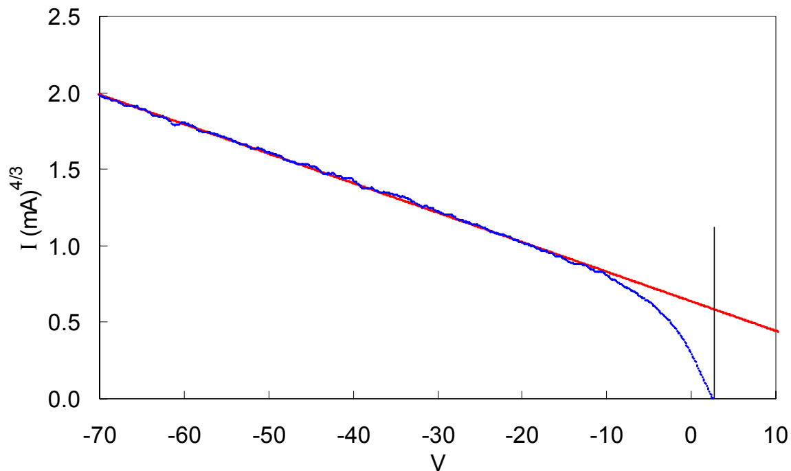
Fig. 4. Ion current I_i^{4/3} vs. V , and a least-squares fitted straight line. The electron current has not been subtracted from the I_i data. The intersection of the line with the vertical line at floating potential V_f yields the value of I_i(V_f) used in the analysis.
