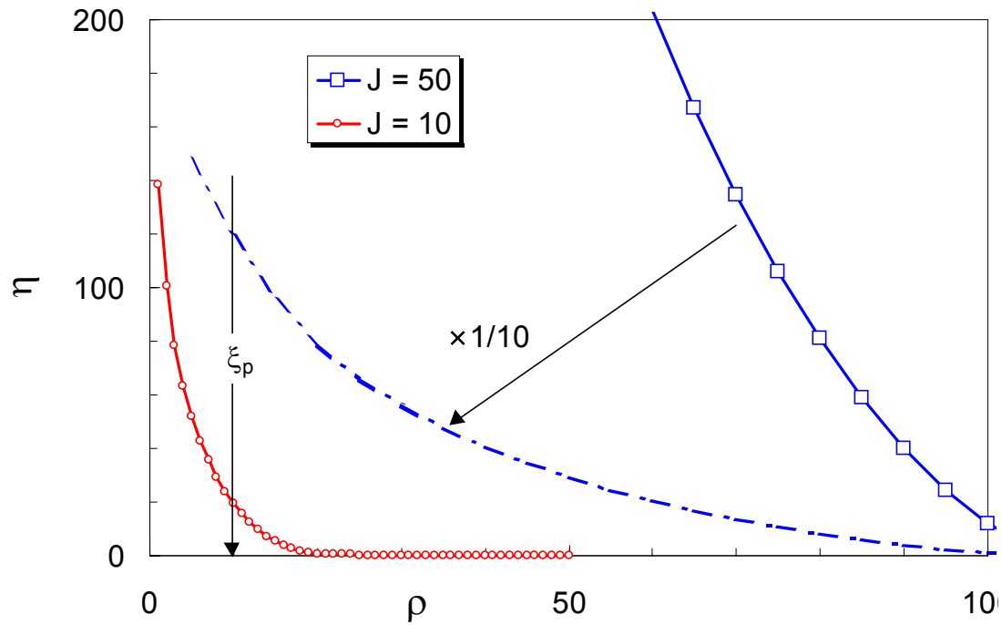
Fig. 9. Potential profiles in a cylindrical sheath for two values of normalized probe current J . The dashed line is the J = 50 curve reduced by 10. The line \xi_p marks the probe radius.
