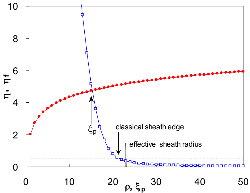
Fig 10. The functions \eta(\xi) and \eta_f(\xi_p) for J = 10 in argon. The “classical sheath edge” is the radius at \eta = 0.5 , where the ions have velocity c_s . The “effective sheath radius” is that at which the assumed probe current would be collected if the Bohm criterion were satisfied there (which it is not).
