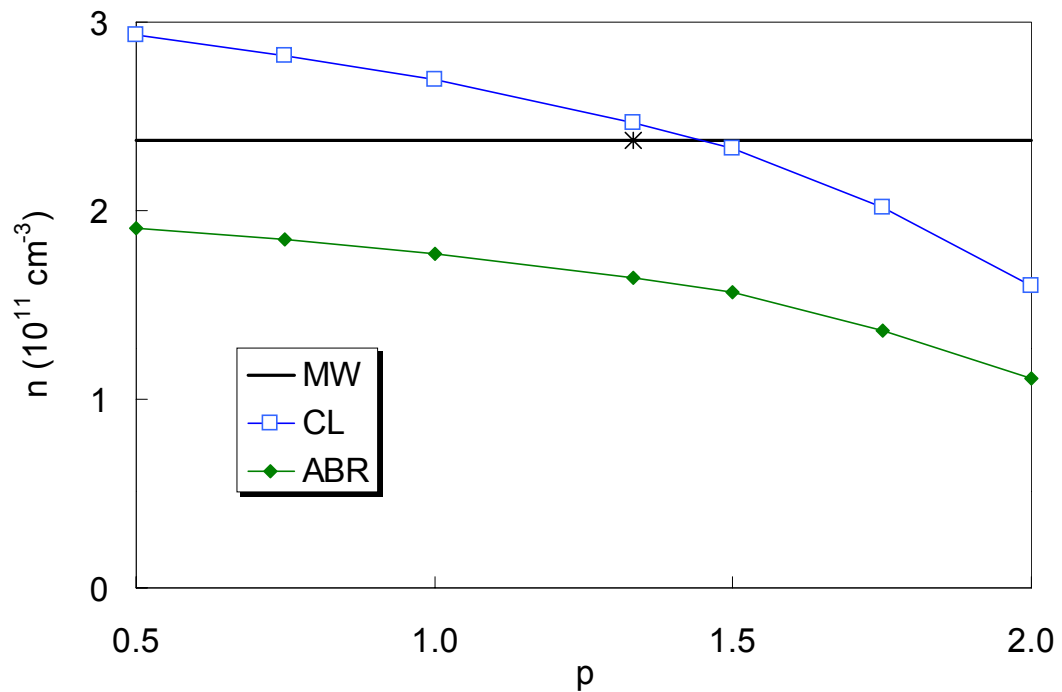
Fig. 14. Dependence of calculated density on the exponent p in I_i^p \propto V_p . Values of n computed with the CL formula and the ABR theory are compared with that measured with microwaves (MW). The star marks the value p = 4/3 .
