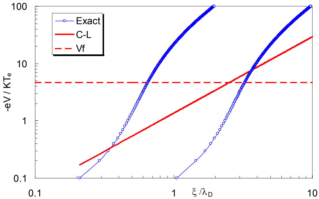
Fig. 7. The two curves of Fig. 6 on a log-log scale, compared with the normalized Child-Langmuir sheath thickness. The dashed line is the floating potential of a plane probe.
