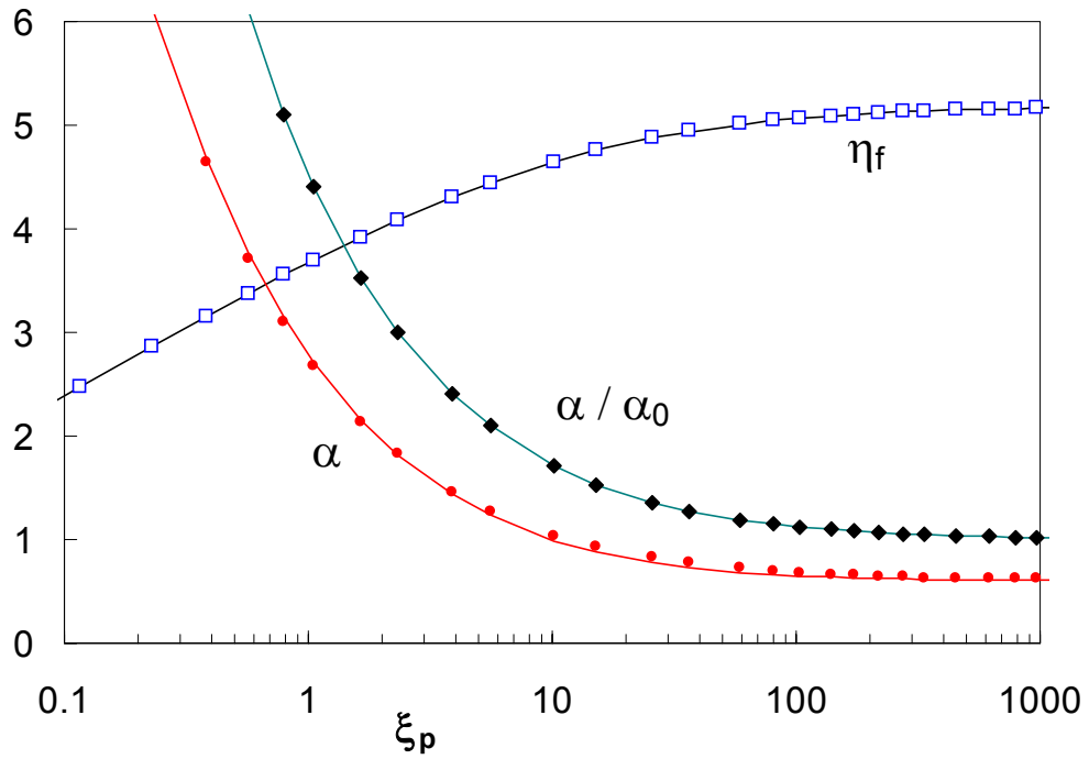
Fig. 11. Computed values of \eta_f = -eV_f / KT_e , \alpha , and \alpha / \alpha_0 for a cylindrical probe in argon and purely radial ion orbits. The curve through the \alpha points is the analytic fit of Eq. (29).
