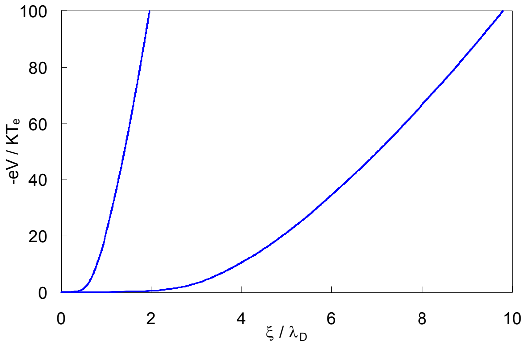
Fig. 6. Calculated potential in a plane sheath with different assumed boundary conditions at the sheath edge \xi = 0 , where V \equiv 0 .
