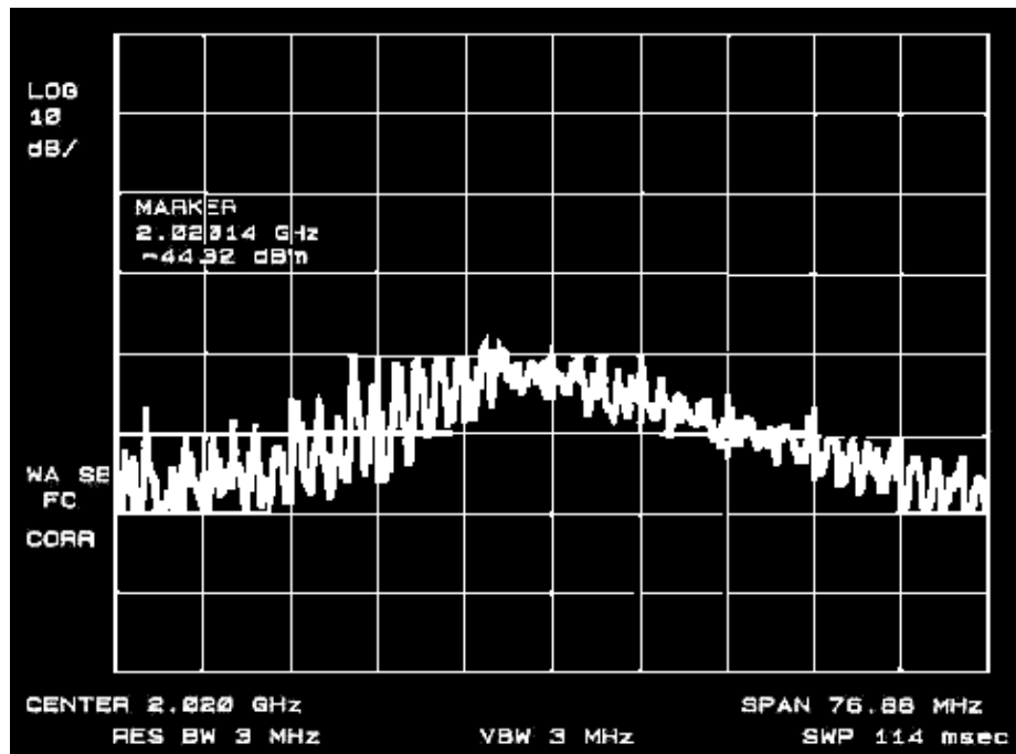
Fig. 16b: Same as (a), but f -scale expanded - sidebands at f_{rf} and harmonics observed.
