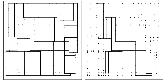
Figure 6: Escape grid reduction for testcase grid.5
