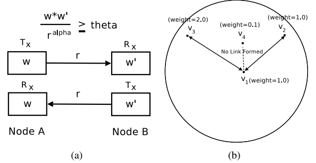
Figure 1. (a) A simple illustration of link formation between two nodes. (b) Irregular coverage: v_1 is not connected to v_4 even though v_4 is very close in distance.
