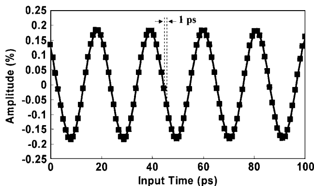
FIG. 3. Digitization of a 48 GHz sinusoid at 1 TSA/s. Lines are obtained using standard sine curve fitting.
