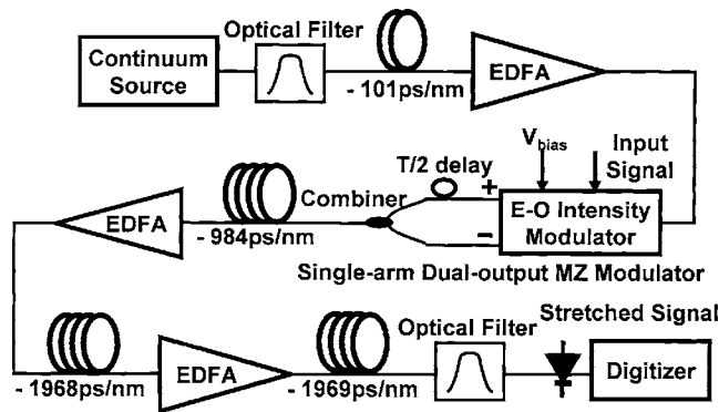
FIG. 2. Experiment setup of TSA/s digitizer with a 50× photonic time stretch preprocessor. EDFA: erbium-doped fiber amplifier.
