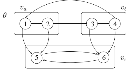
Figure 2: Safety game, with objective \Box T for T = \{1, 2, 3, 4\} .
