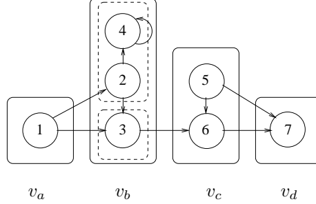
Figure 1: Three-Valued Abstraction Refinement in Reachability Game
