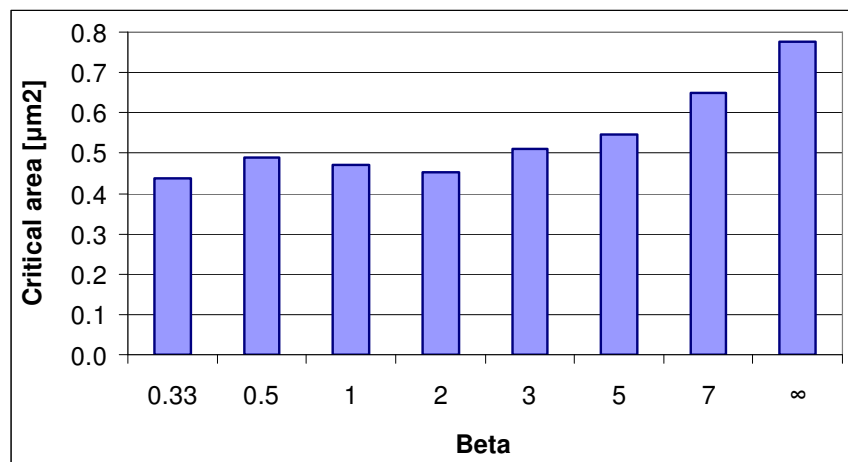
Figure 4.7. Critical area for metal layer 2 of generated layouts with different \beta .
