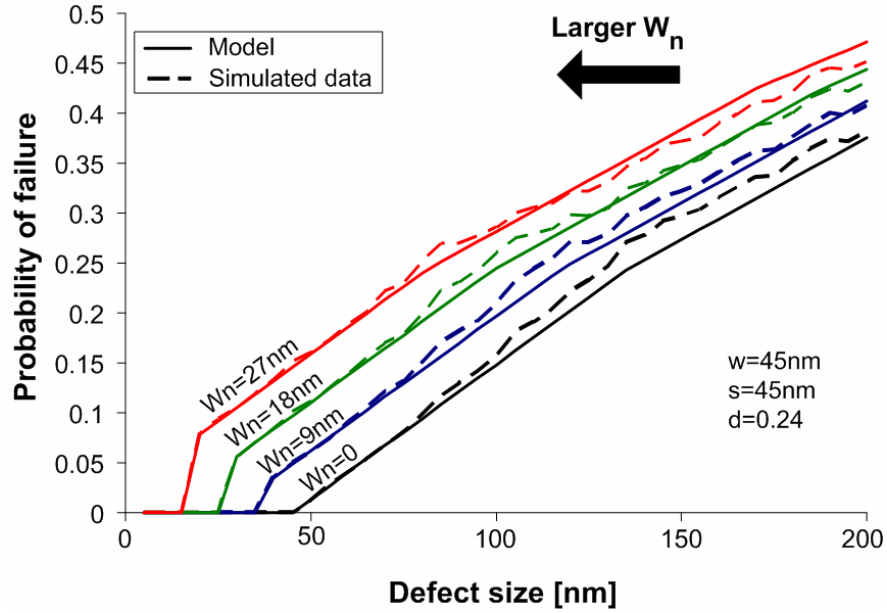
Figure 5.7. Comparison of modeled and simulated probabilities of failure due to open and narrow defects for different critical widths, w_n .
