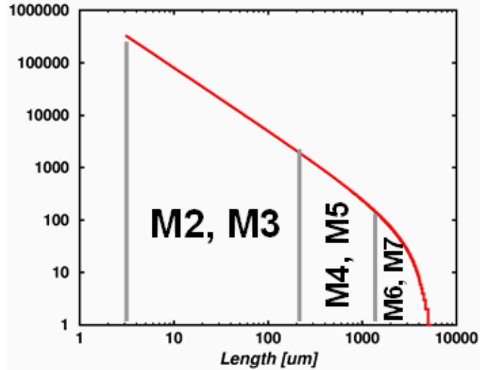
Figure 4.3. idf for a real design of 75 million gates and 55.6 million nets and metal layer allocation based on wire lengths.
