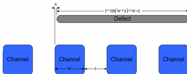
Figure 3.1. An example of an open defect covering 2 channels.
