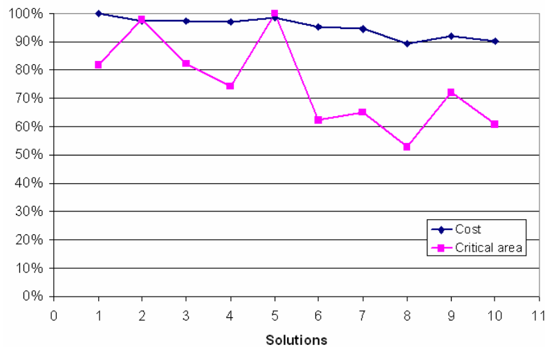
Figure 4.1. Comparison of normalized costs and critical areas of different solutions found by PRS
