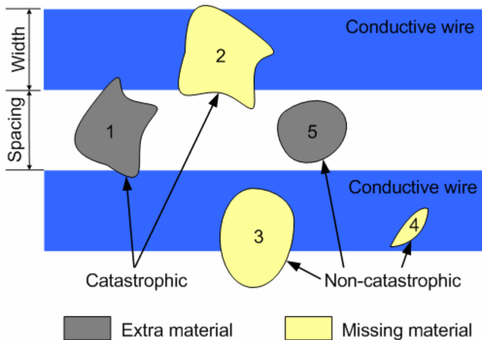
Figure 2.1. Missing vs. extra material and catastrophic vs. non-catastrophic defect classifications.
