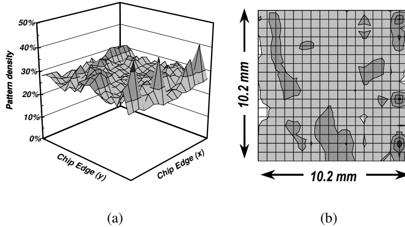
Figure 3.11. Pattern density distribution in 3D (a), and in 2D (b).
