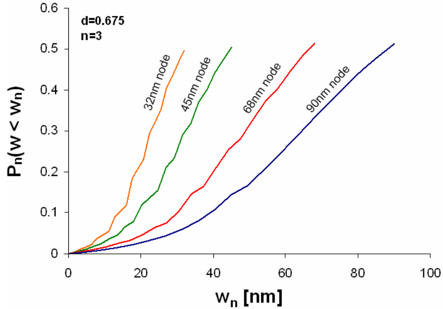
Figure 5.8. Plots of probability P_n of formation of an open or narrow as a function of the critical width, w_n , for 90nm, 68nm, 45nm, and 32nm technology nodes.
