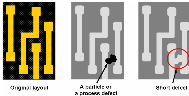
Figure 2.3. Sample of a layout showing a short defect.
