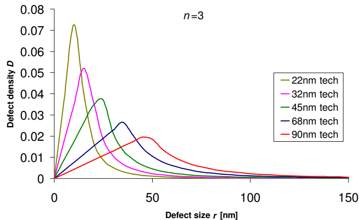
Figure 3.8. Defect size distribution for 90, 68, 45, 32, and 22nm technology nodes in a typical fabrication line.
