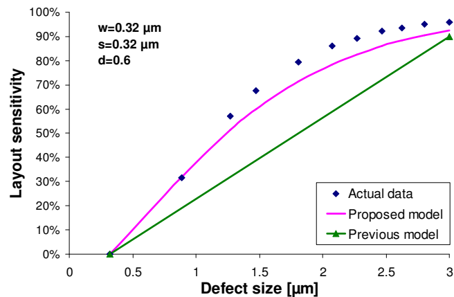
Figure 3.4. Comparison of the proposed sensitivity model with extracted layout sensitivity and a previous sensitivity model [41] for short defects.
