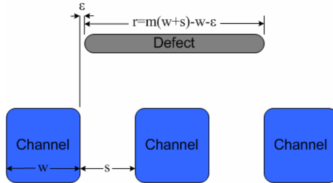
Figure 3.2. An example of a short defect covering 2 channels.
