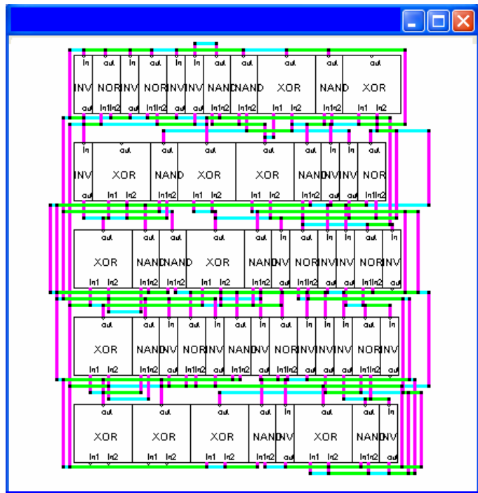
Figure 4.5. Output display of YA-PRS when run on real design of 52 gates
