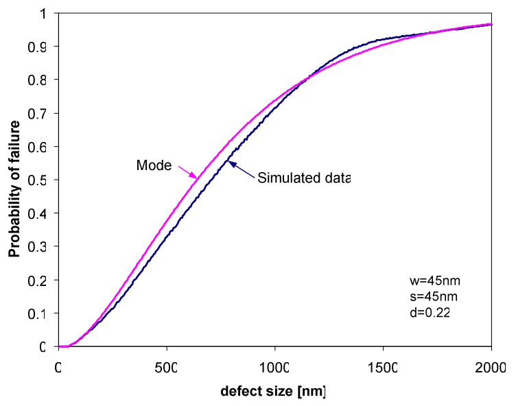
Figure 3.7. Comparison between probability of failure estimated by the layout sensitivity model for short defects and probability of failure due to short defects extracted from an actual design.
