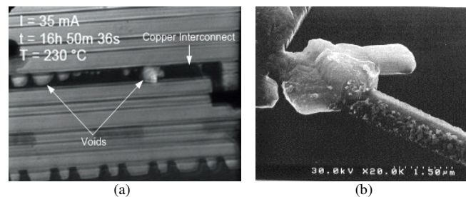
Figure 5.2. Examples of EM induced failure. (a) Open circuit resulting from formation of voids due to EM in a line interconnect [76]. (b) Extrusion of metal through the passivation layer [77].
