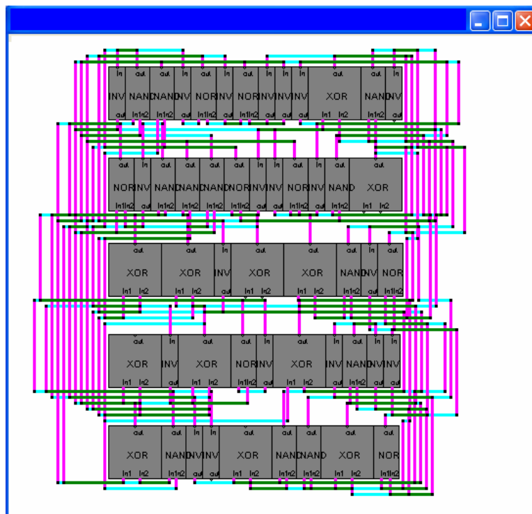
Figure 5.6. PRS displaying the layout of a circuit that computes the absolute value of the difference between two 2-bit numbers.
