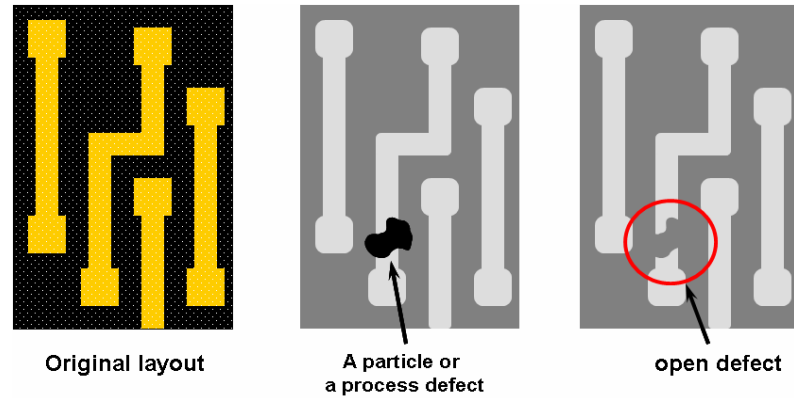
Figure 2.2. Sample of a layout showing an open defect
