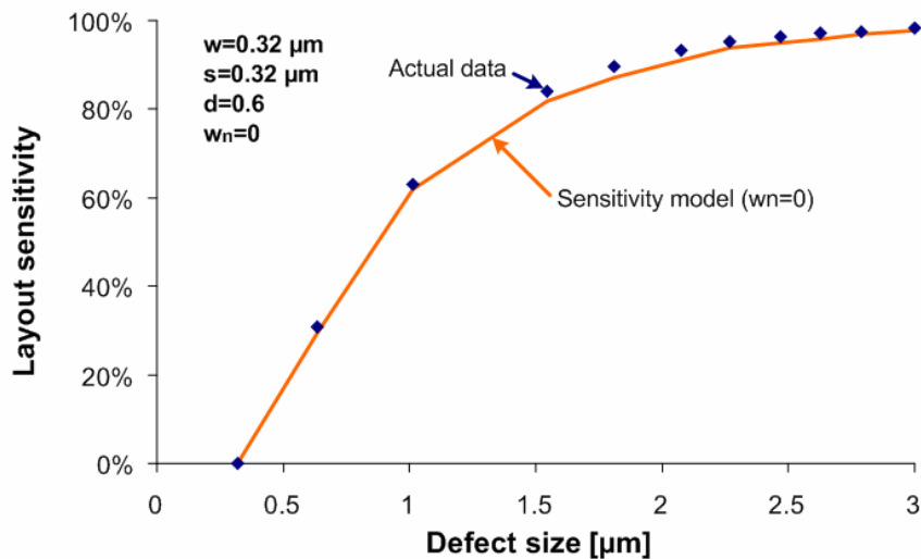
Figure 5.5. Comparison of sensitivity model with actual extracted layout sensitivity for open defects.
