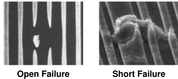
Figure 2.4. Spot defect photographs (Photograph used with permission of EE Times , a CMP Media LLC publication) [20].
