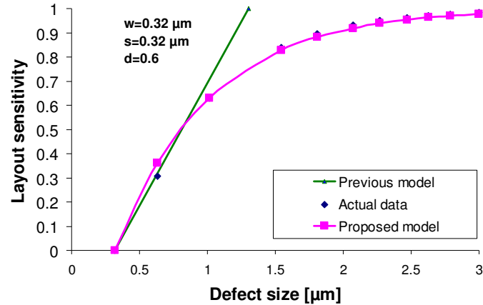
Figure 3.3. Comparison of the proposed sensitivity model with extracted layout sensitivity and a previous sensitivity model [41] for open defects.
