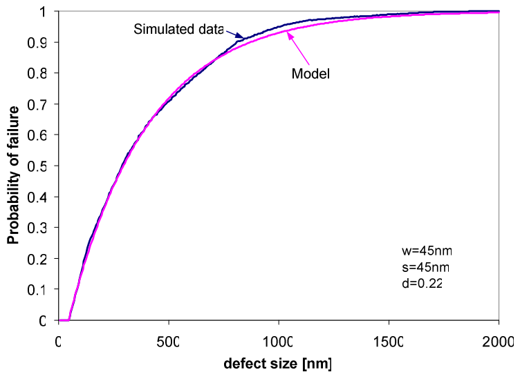
Figure 3.6. Comparison between the probability of failure estimated by the layout sensitivity model for open defects and probability of failure due to open defects extracted from an actual design.
