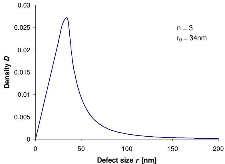
Figure 2.7. Defect size distribution for 65nm technology nodes in a typical fabrication line.
