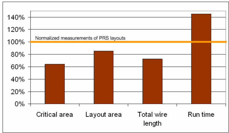
Figure 4.6. Comparison of average critical area for metal layer 2, layout area, total wire length, and run time for layouts generated by PRS and YA-PRS.
