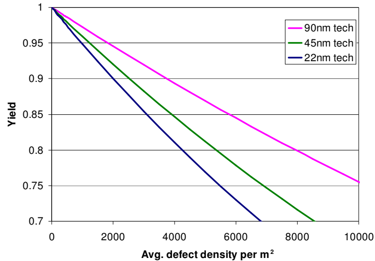
Figure 3.10. Plot of manufacturing yield as a function of average defect density for 90, 45, and 22nm technology nodes.
