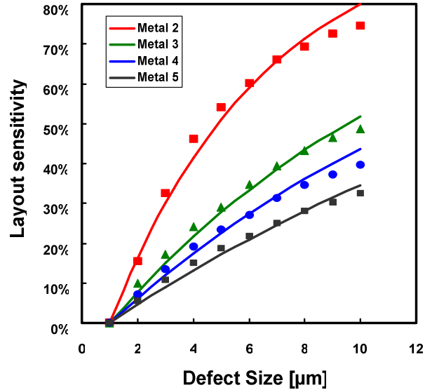
Figure 3.5. Comparison of the proposed model with layout sensitivity for shorts extracted from a real micro-processor chip [44].
