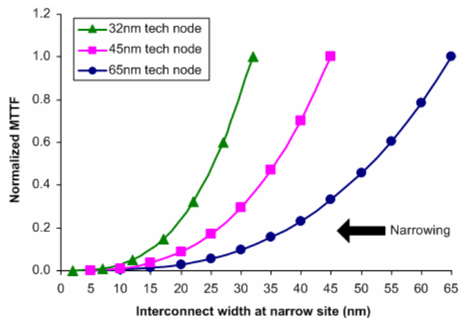
Figure 5.3. Plot of normalized MTTF vs. interconnect width at narrow site for 65nm, 45nm, and 32nm technology nodes.
