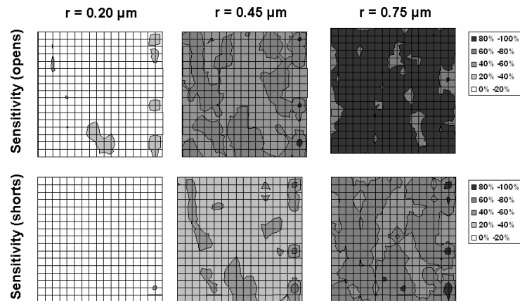
Figure 3.12. Layout sensitivity patterns in a real design using the proposed layout sensitivity model i.e. equations (3.5) and (3.12).
