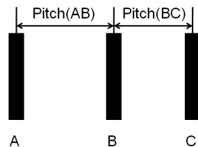
Figure 2: Example illustrating gate-pitch restriction. In case Pitch(AB) is < X_0 but different than X , then Pitch(BC) is restricted to either X or \geq X_0 . The same restriction applies to Pitch(AB) if Pitch(BC) is unrestricted.
