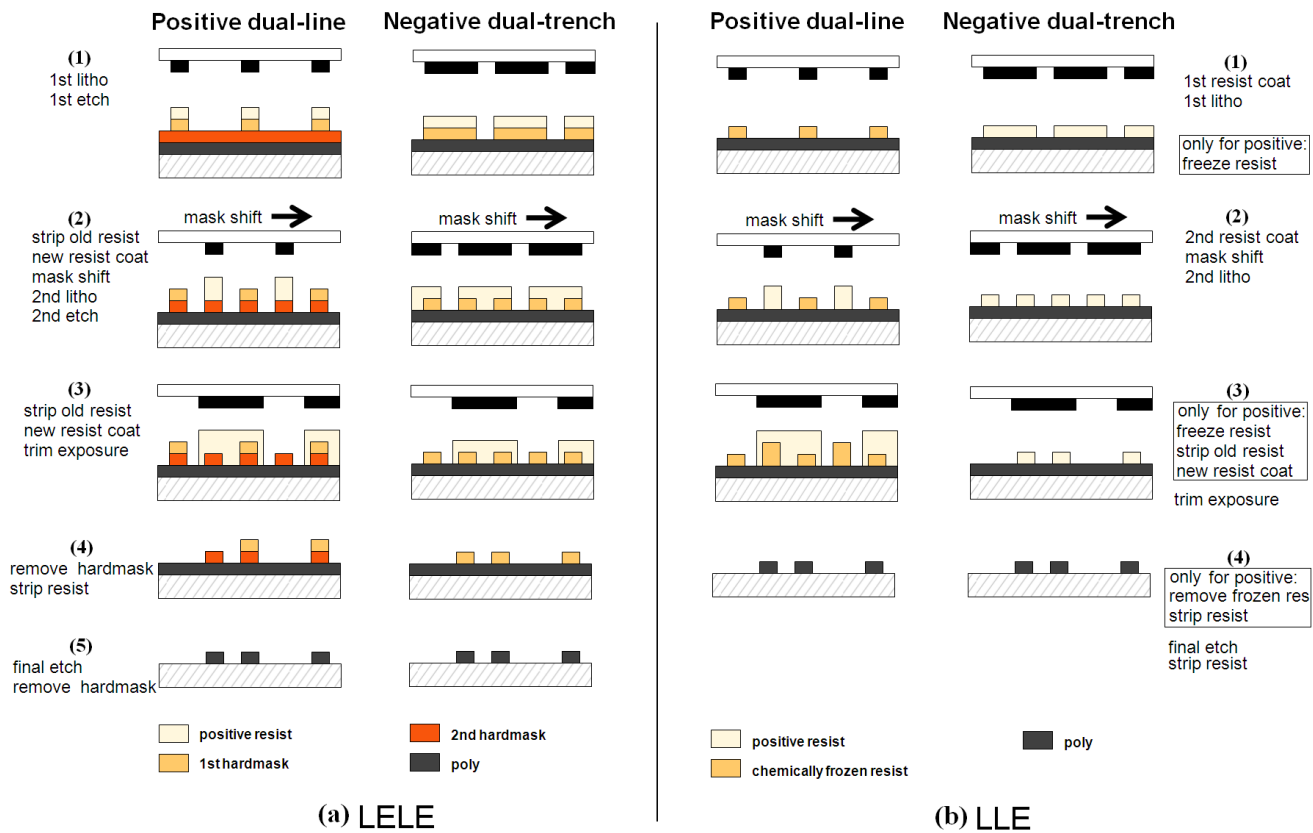
Figure 1: Proposed manufacturing processes for ST-DPL: (a) LELE and (b) LLE positive dual-line and negative dual-trench processes.
