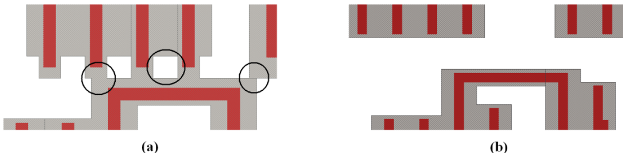
Figure 6: Trim-mask complexity at cell-boundaries before (a) and after (b) including rules (2) and (3).
