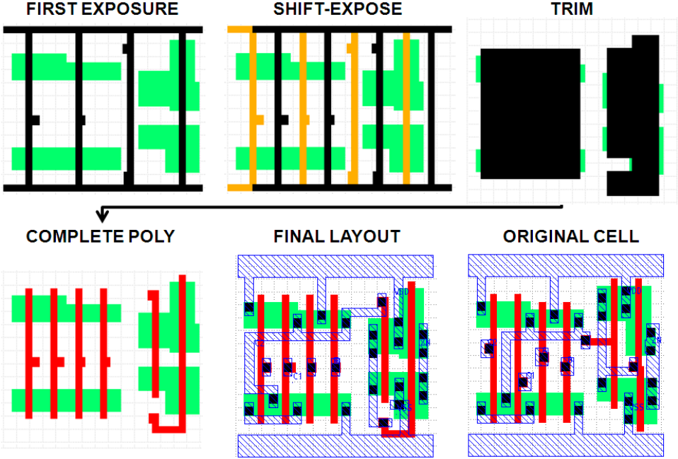
Figure 4: Example of 4-input OAI cell layout migrated for the application of ST-DPL.
