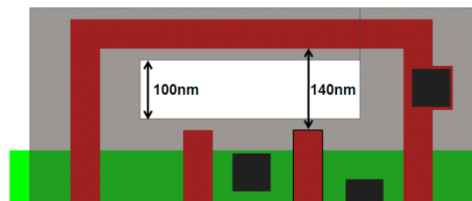
Figure 5: Poly line-tip to poly side spacing rule of 140nm to ensure a minimum hole width of 100nm.
