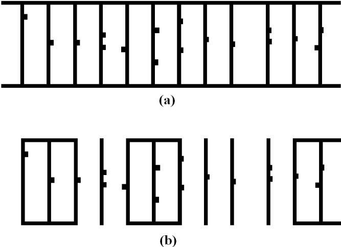
Figure 3: ST-DPL critical mask snippet corresponding to a flip-flop cell with two structure-options (a) and (b).
