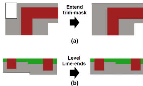
Figure 7: Trim-mask notch-fill by (a) trim-mask extension and (b) poly line-end leveling.
