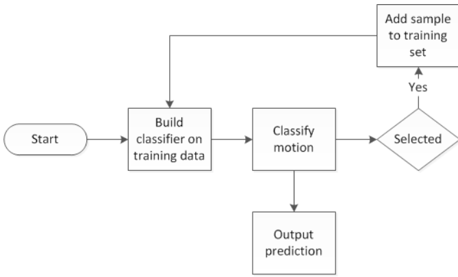
Fig. 1. Classifier improvement
