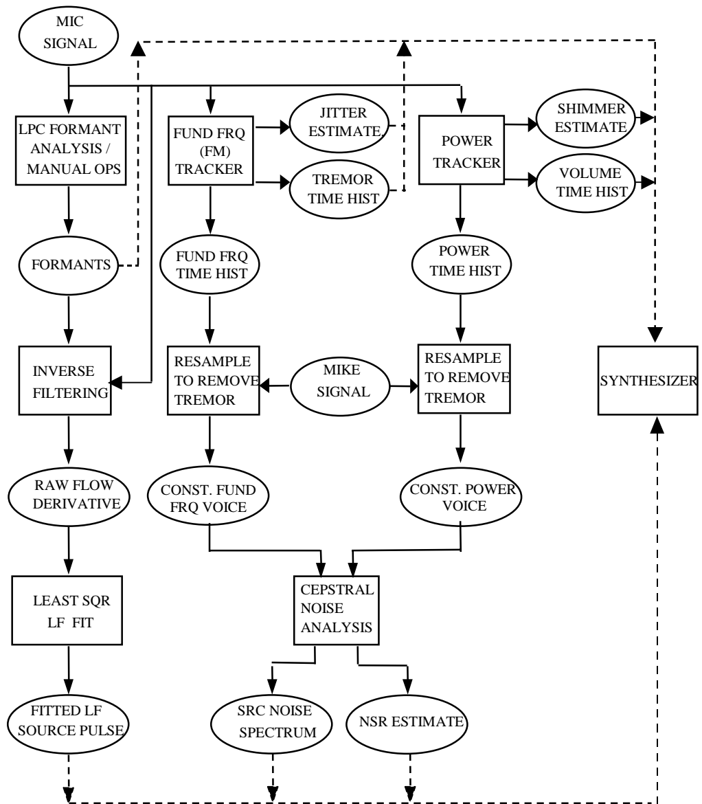
Figure 2.1. Overall voice analysis/synthesis steps. Details are omitted for clarity. Analysis (solid lines) steps include LPC formant analysis, inverse filtering, source fitting, fundamental frequency tracking, power tracking, jitter estimation, shimmer estimation, and source aspiration noise estimation. Results are input to the synthesizer (dashed lines).
