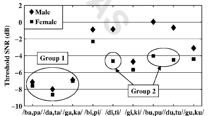
FIG. 7. Threshold SNR values (dB) for the nine voiced/voiceless pairs, separated by gender of the talkers. Group 1 (/Ca/ syllables) shows little difference in perceiving male versus female tokens, while Group 2 (/di, ti/, /du, tu/, and /bu, pu/) shows large gender related differences.
