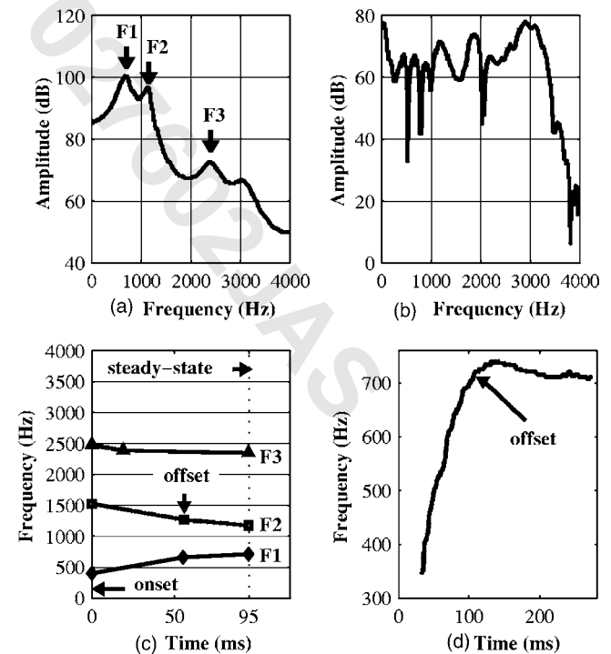
FIG. 2. (a) LPC spectrum of a /t a/ token during the vowel, (b) DFT spectrum of a /t a/ token during the burst, (c) formant transition measurements, and (d) determination of formant transition offset (with the F1 frequencies obtained from an 8 kHz wave form using LPC analyses).
