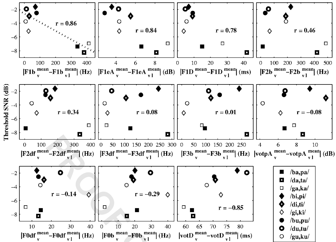
FIG. 8. Threshold SNRs and absolute differences of the means of several acoustic properties for the nine voiced/voiceless pairs. For each point (CV pair), the threshold SNR and the difference of the means resulted from the perception and measurement of 32 tokens (four talkers \times four tokens of the same syllable \times two syllables in one CV pair), respectively. Each point is indicated with its vowel context [ /a/ (square), /i/ (diamond), or /u/ (circle)] and place of articulation [ /b, p/ (solid), /d, t/ (bold), or /g, k/ (thin)]. Numbers inside panels are the correlation coefficients between the nine threshold SNRs and the nine absolute differences of the means. A fitted line is shown in only one panel for illustrative purposes.
