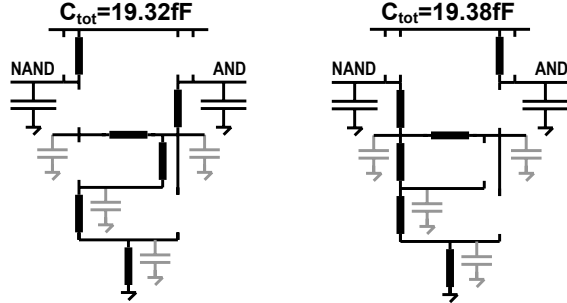
Fig. 4. Discharge event of SABL AND-NAND gate in the evaluation phase for (0,1)-input (left); and (1,1)-input (right).
